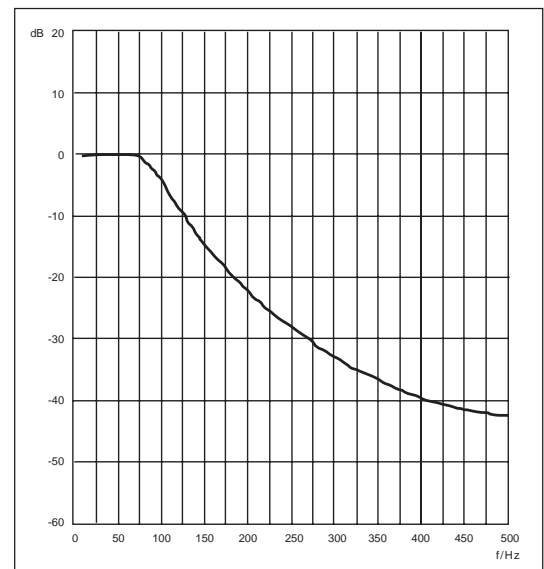
Fig. 2. Filter characteristics of the measuring input of the earth-fault current for SPCJ 4D29.
