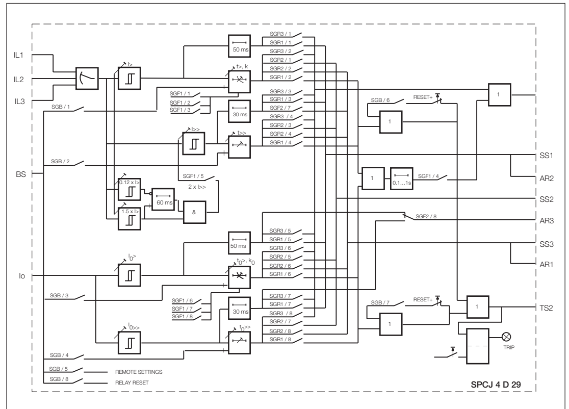
Fig. 3. Block diagram for the combined overcurrent and earth-fault relay module SPCJ 4D29.
