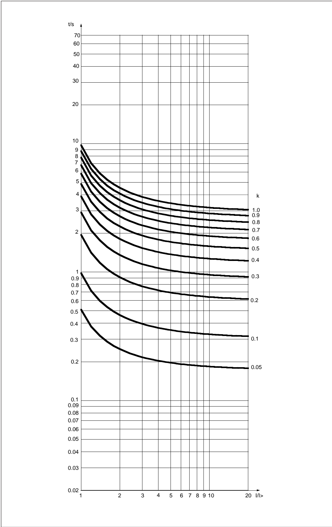
Fig. 9. RI-type inverse-time characteristics of the overcurrent and earth-fault unit SPCJ 4D29.
