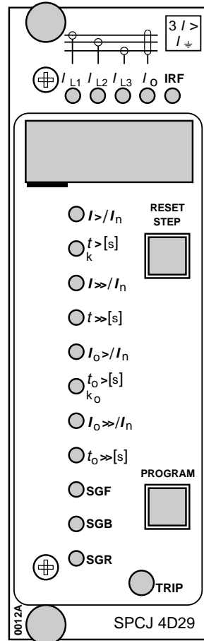
Fig. 4. Front panel of the combined overcurrent and earth-fault relay module SPCJ 4D29.
