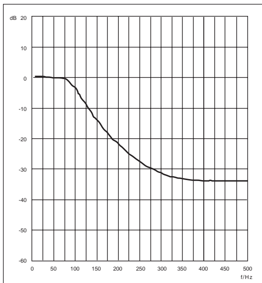
Fig. 1. Filter characteristics of the measuring inputs of the overcurrents for SPCJ 4D29.
